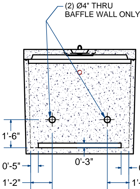
VIEW BAFFLE WALL
